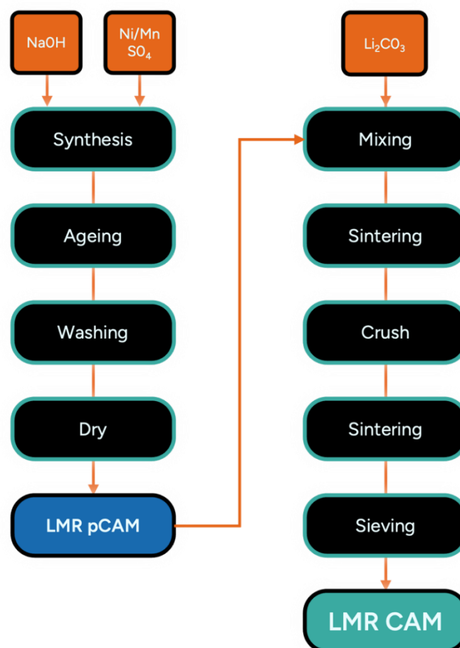
Figure 8: Firebird's LMR CAM production process flow.
